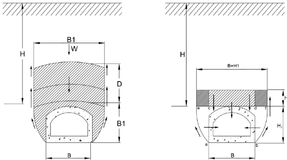
Fig. 2: Arc formation process in tunnel and its loads
