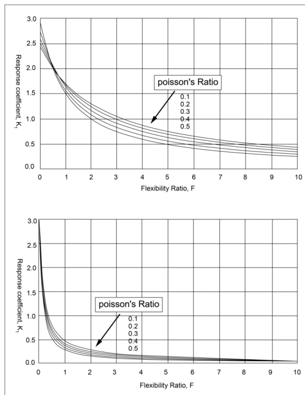
Fig. 4: coverage response factor versus flexibility ratio of full slip condition (circular tunnel)
