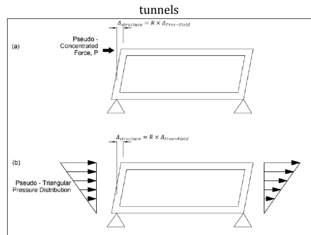
Fig. 7: Simplified frame model of tunnel (a) quasi-concentrated load for deep tunnel (b) quasi-triangular pressure for shallow tunnel
