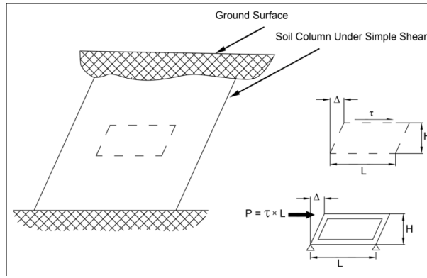
Fig. 5: Soil relative stiffness and a rectangular frame
