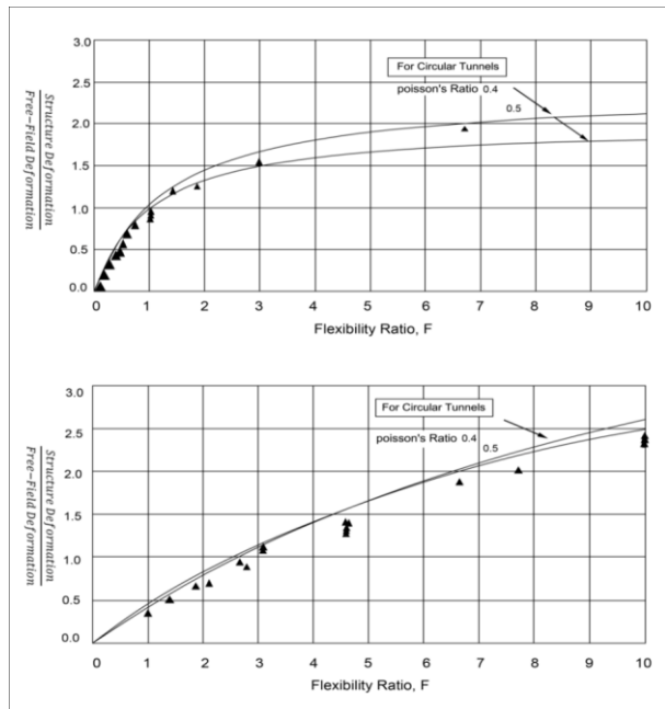
Fig. 6: Comparison of dimensionless structural deformation versus flexibility ratio of rectangular and circular
