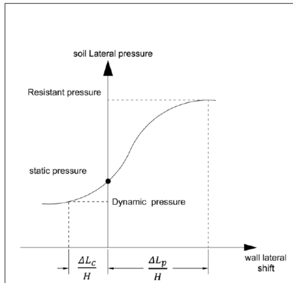
Fig. 1: Soil lateral displacement versus structure displacement
