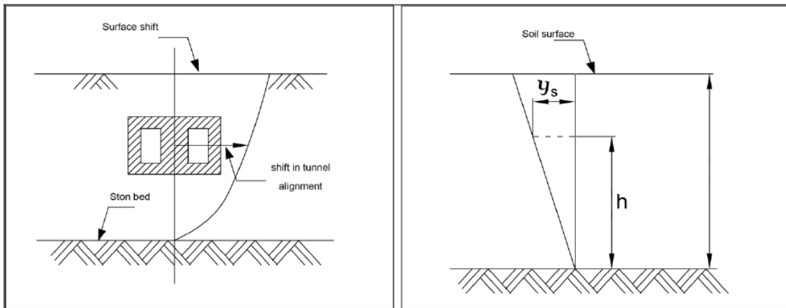
Fig. 3: deformation of underground structure regarding to its distance from bedrock ratio
